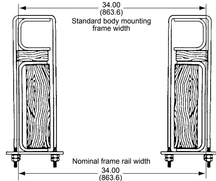
FIGURE 9 Frame rail and body mounting frame widths
