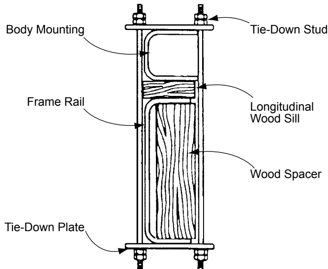
FIGURE 8 Typical attachment with hardwood spacer
