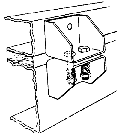
FIGURE 6 Spring loaded attachment
