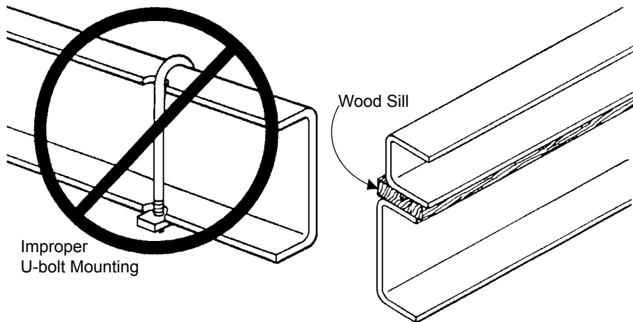
FIGURE 1 U-bolt on notched side rail can cause premature failure of frame rail
