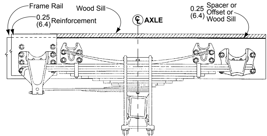
FIGURE 3 Frame rail with 1/4" Outsert
