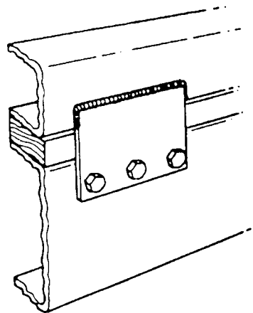
FIGURE 5 Rigid Mount
